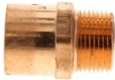
1-1/4" Female Copper Solder x 1" Male NPT Adapter
